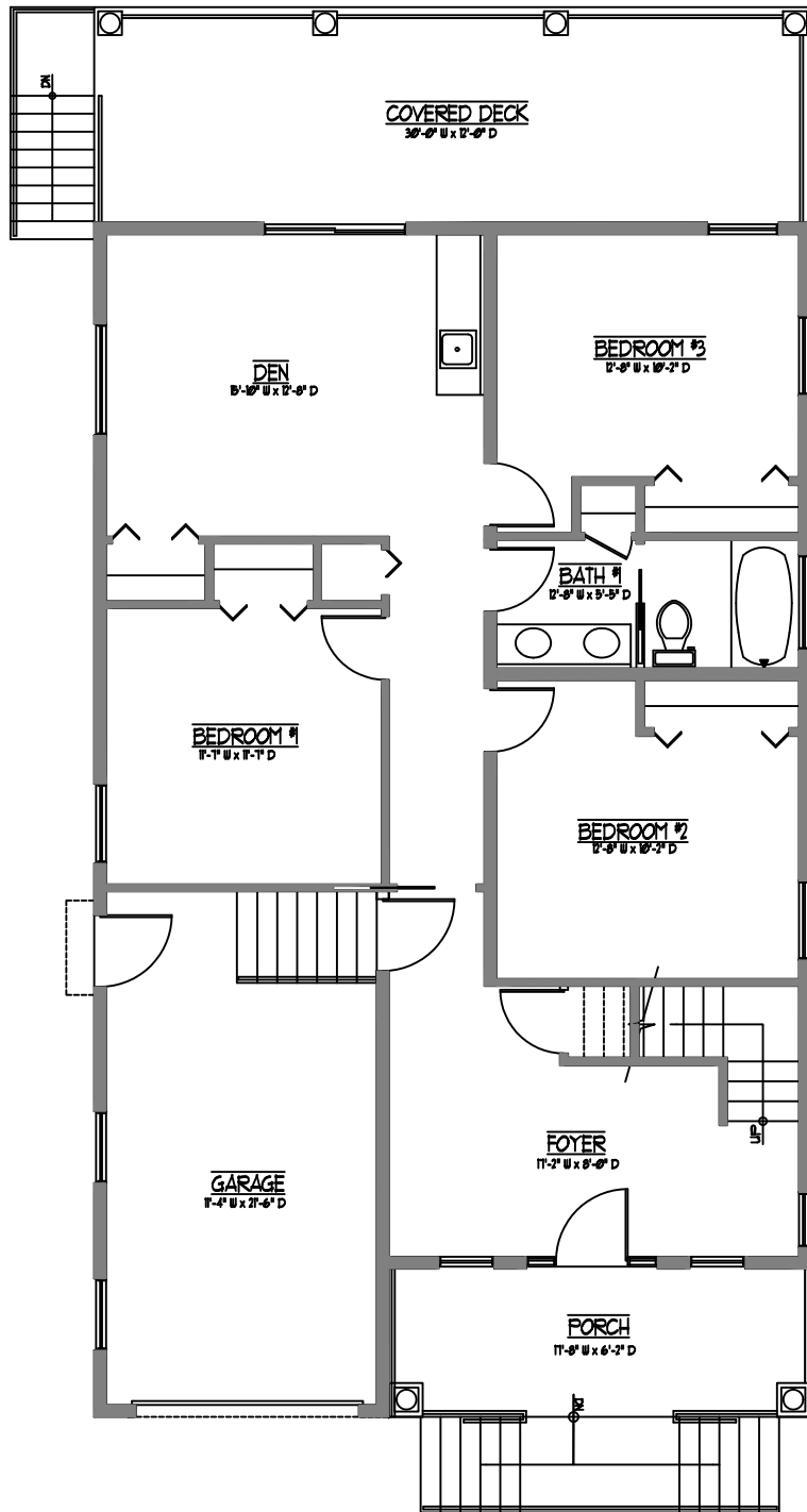
① FIRST FLOOR PLAN 1/4" = 1'-0"
